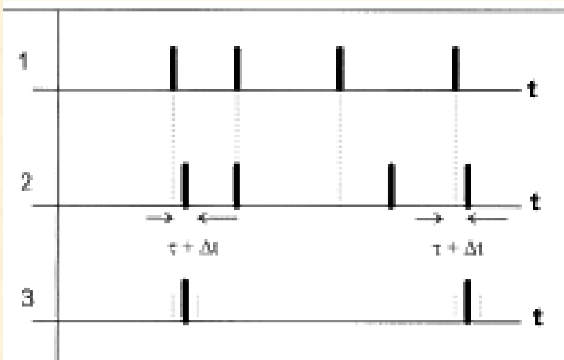
Figure 3 Coincidence counting of biophotons, where at least one photon in Channel '1' has to be registered in a time interval t < \tau < t + \Delta t before a registered photon in Channel '2'.
