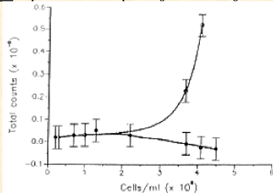
Figure 5b Delayed luminescence of cancer cells (upper curve) and normal cells (lower curve) in dependence on the cell density.
