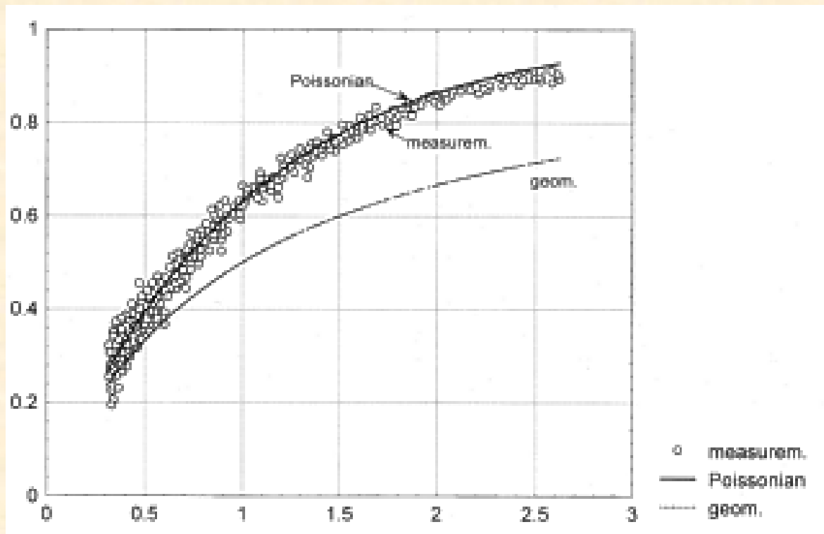
Figure 4a Agreement of the Poissonian distribution with the PCS of biophoton emission of a leaf. The value Z_j/n_{2j} is displayed in dependence on 1_{2j}.dt .
