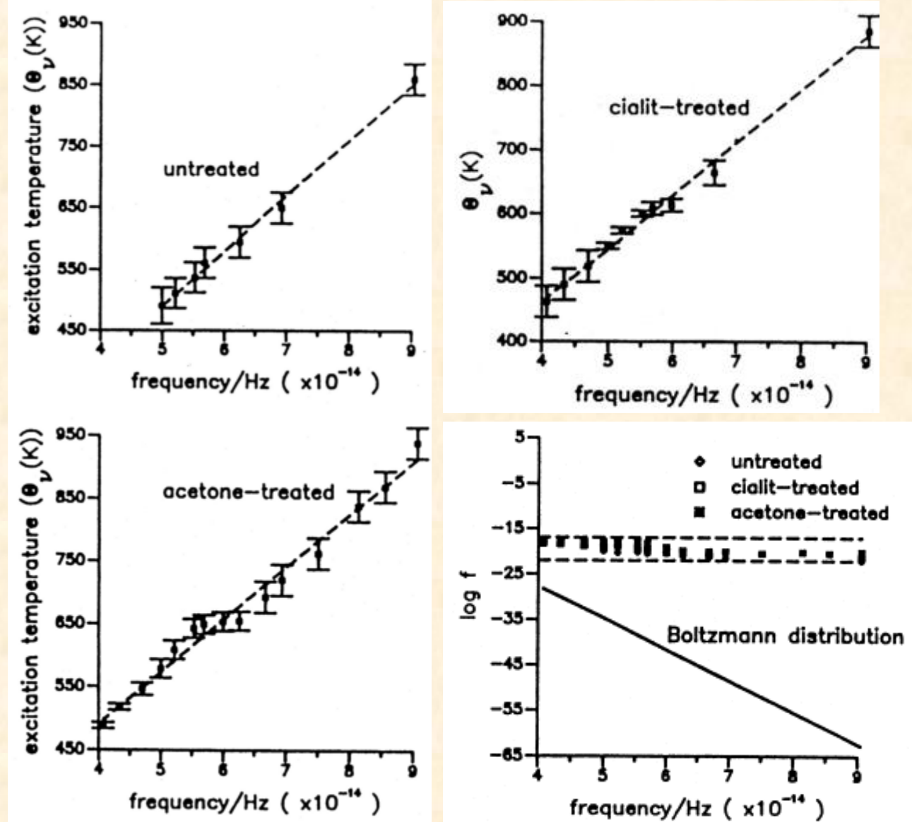
Figure 1: Excitation temperature \theta(v) = h v / k \ln(2v^2 F / c^2 n v) of cucumber seedlings under different treatments and the \ln(f(v)) -value compared to the Boltzman \ln(f(v)) .
