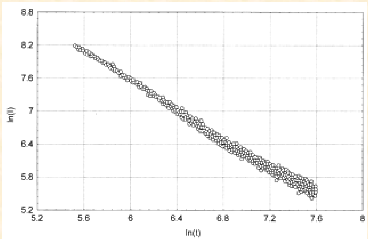
Figure 4b Relaxation of the leaf of Figure 4a , where the logarithm of the intensity is displayed versus the logarithm of the time.
