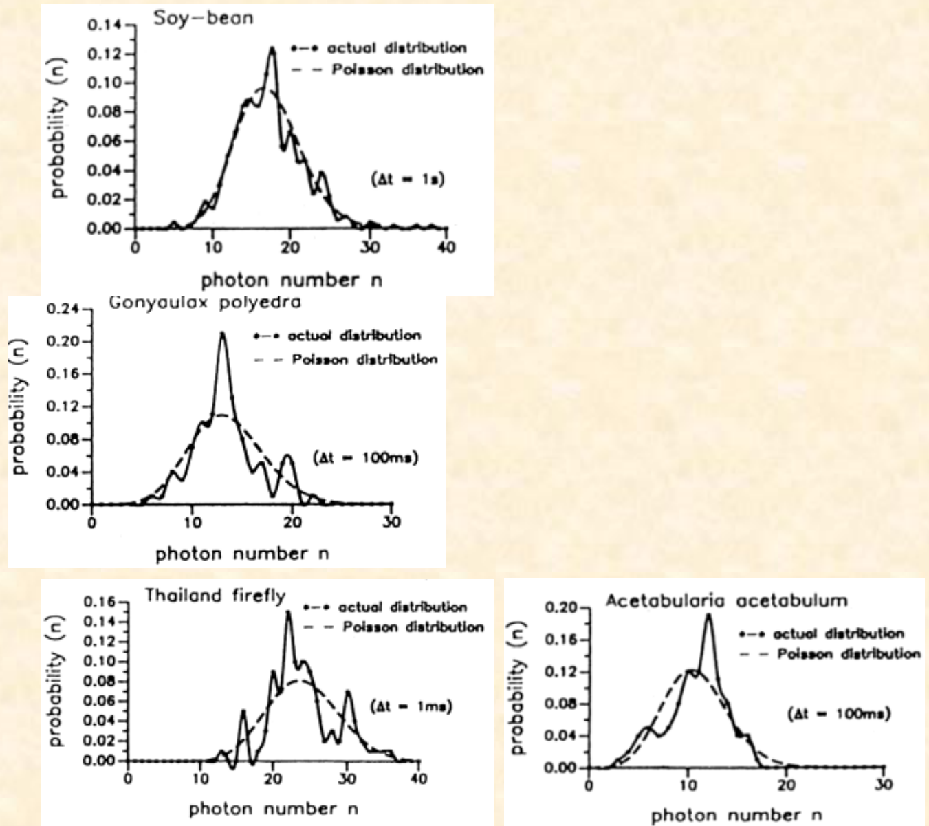
Figure 2: Agreement of the Photocount Statistics of different biological systems with a Poissonian distribution.
